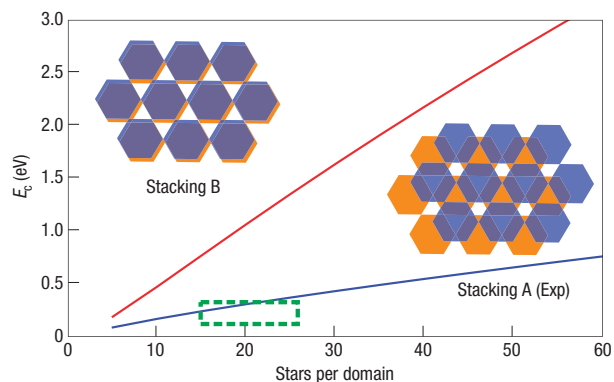
Figure 4 The results for the Coulomb energy calculation for two different domain stackings as a function of domain size. The lower line (blue) corresponds to an axial arrangement of domains (hexagonal) and interdomain spaces (triangular) between adjacent layers (stacking A), as deduced from experiment 27 ; the upper line (red) shows for comparison, the Coulomb energy for a hypothetical axial domain stacking between successive layers (stacking B). The green dashed rectangle depicts the values of domain sizes that were experimentally observed in the NCCDW phase at ambient pressure. We note that the Coulomb energies calculated for these values are comparable to the energy of the gap, hinting at a possible Coulomb-controlled phase separation.
