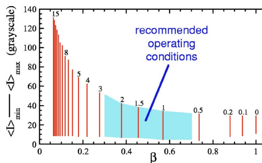
FIG. 9. Recommended average intensity levels for an 8-bit digital camera, as a function of the intercept \beta = v_2(0) ; the corresponding pixel area is labelled in units of average speckle area. If the average intensity is too low, then error occurs due to digitizing the intensity crudely into a small number of bins. If the average intensity is too high, then error occurs due to clipping of the high-intensity tail of the distribution. The vertical bars indicate the range over which these effects cause less than a 0.1% error in the variance. For n -bit cameras, the lower limit does not change but the upper limit scales with the number of grayscale levels.
