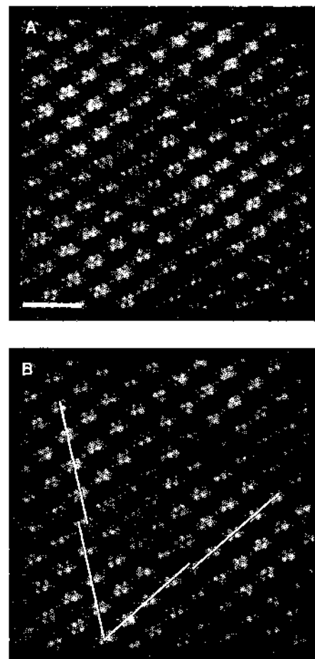
Fig. 3. (A) Atomic resolution raw data of 1T-TaS 2 recorded with a tunneling current of 2 nA and a bias voltage of 10 mV. The domains are located near the four corners of this image. The bar is 25 \text{ \AA} . (B) Low-pass filtered data from (A). Lines have been drawn through three adjacent domains to highlight the one-lattice-period phase shift.
